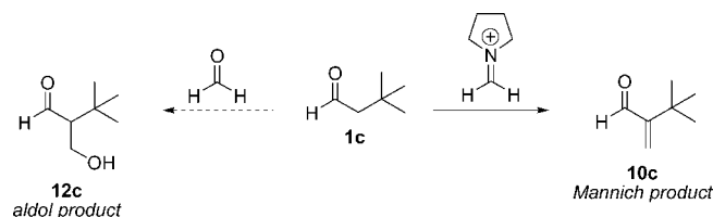
Scheme 2. Competing reaction pathways with 1c .
