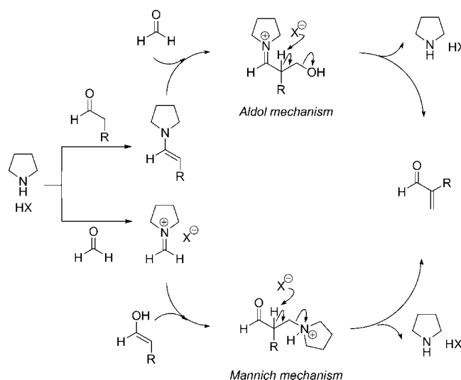
Scheme 1. Possible mechanisms for the \alpha -methylenation reaction.
