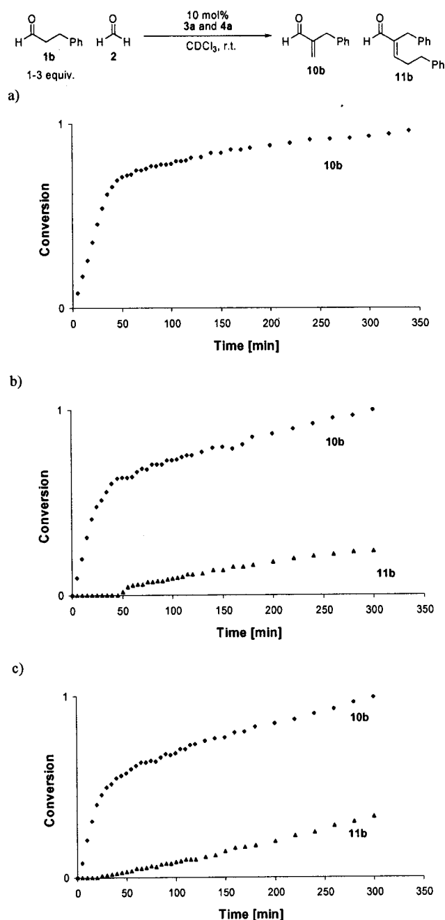
Figure 5. Competition experiment with a) 1:1, b) 2:1, and c) 3:1 ratio of hydrocinnamaldehyde ( 1b )/formaldehyde ( 2 ).
