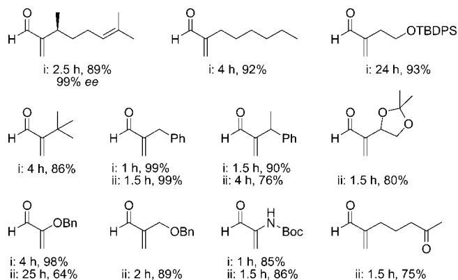
Figure 1. The scope of first- and second-generation catalyst systems.
