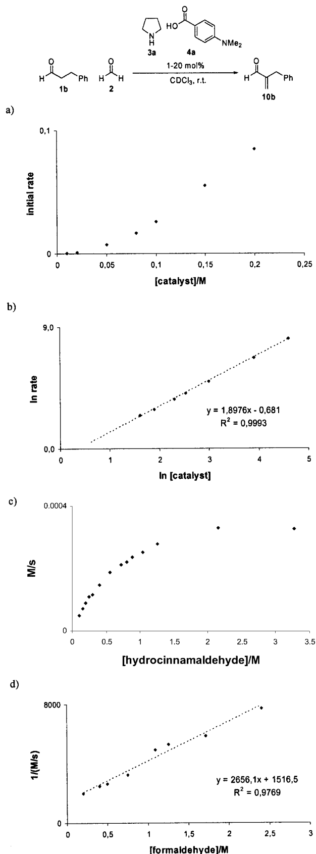
Figure 7. a), b) Second-order dependence of the reaction rate on catalyst concentration, c) saturation kinetics observed with aldehyde 1b , and d) inverse rate relationship observed with formaldehyde. All rates were determined by ^1\text{H} NMR spectroscopy using the method of initial rates (see Supporting Information for details).
