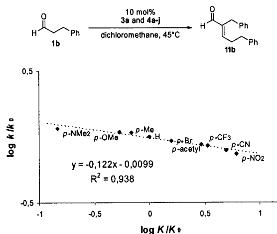
Figure 4. Correlation of benzoic acid dissociation constants with reaction rates of self-condensation of hydrocinnamaldehyde.
