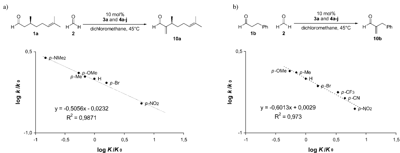
Figure 2. Correlation of benzoic acid dissociation constants with reaction rates of \alpha -methylenation of a) citronellal ( 1a ) and b) hydrocinnamaldehyde ( 1b ).
