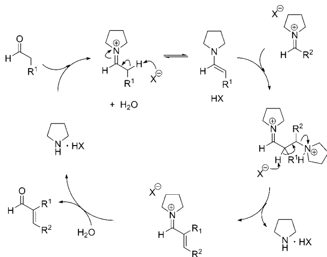
Scheme 3. Double activation of the reaction components by an enamine/iminium mechanism.
