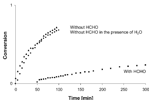
Figure 6. Self-condensation of hydrocinnamaldehyde ( 1b ) to 10b in \text{CDCl}_3 a) under standard conditions, b) in the presence of \text{H}_2\text{O} , c) in the presence of formaldehyde (ratio 1b /formaldehyde = 2:1).
