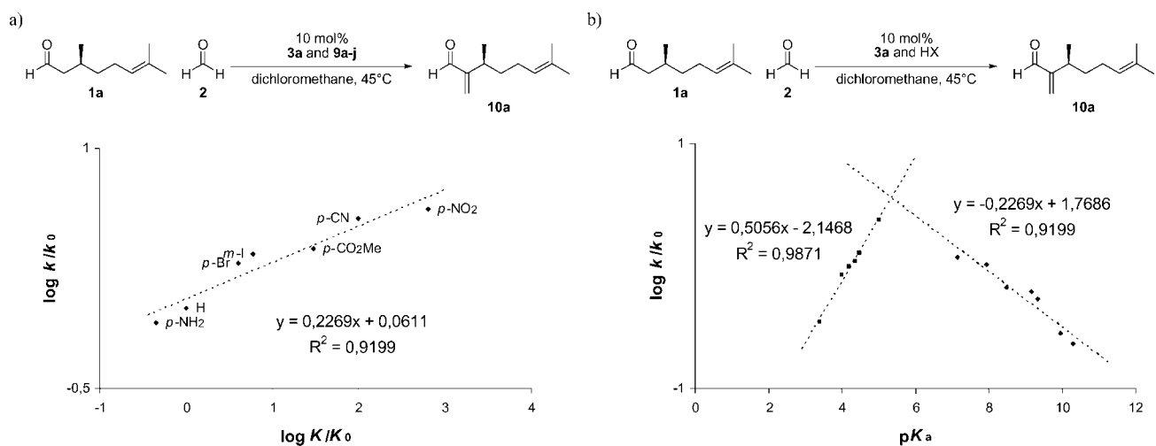
Figure 3. a) Correlation of phenol dissociation constants with reaction rates of \alpha -methylenation of citronellal ( 1a ) and b) comparison of benzoic acids and phenols as co-catalysts, plotted against pK_a of the acid.
